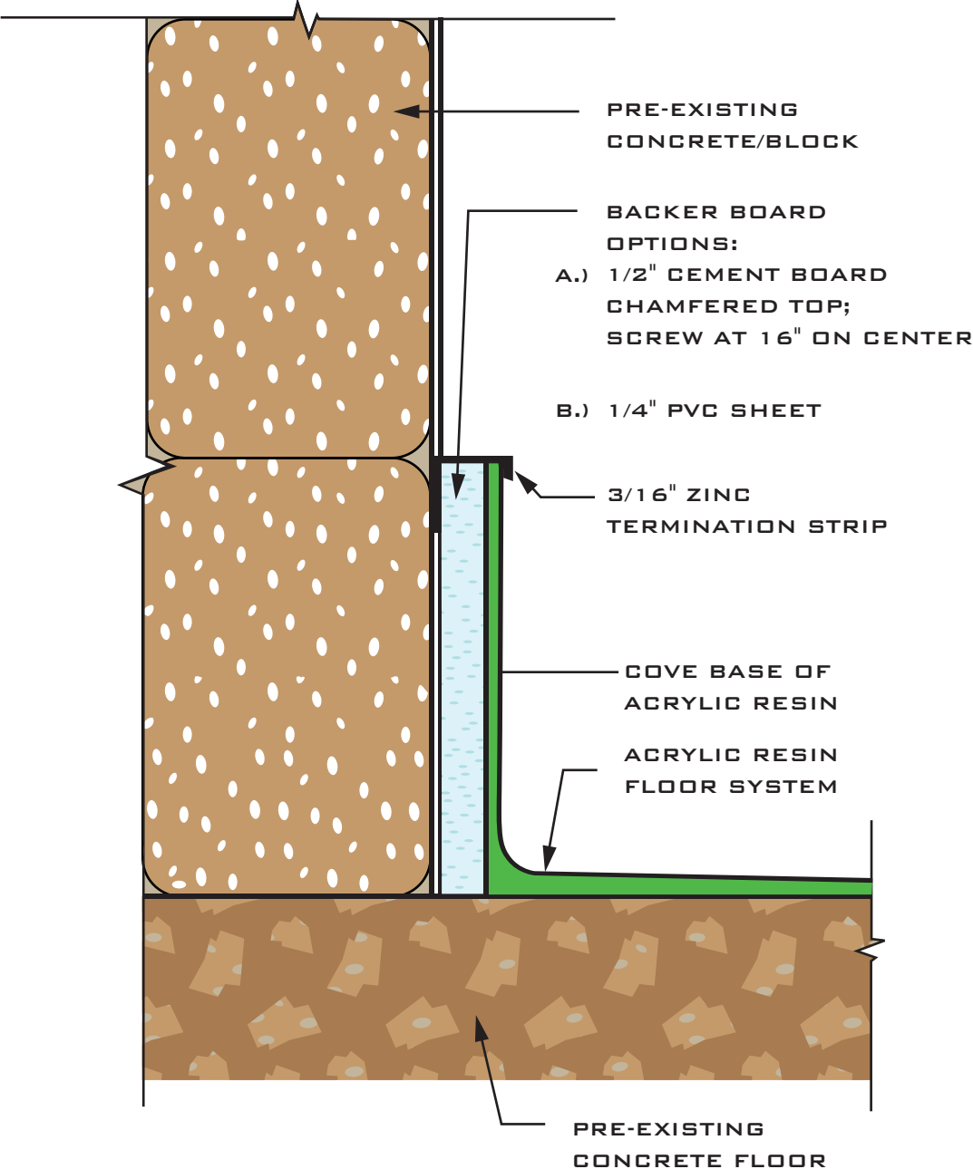
FIGURE B.2 COVE BASE ON CONCRETE/BLOCK SCALE: 6" = 1' - 0"
