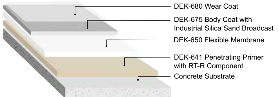
DEK-650 Flexible Membrane achieves 400% elongation as performed by ASTM D638.
