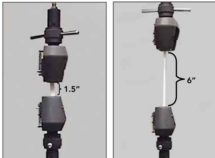
DEK-650 Flexible Membrane achieves 400% elongation as performed by ASTM D638.
