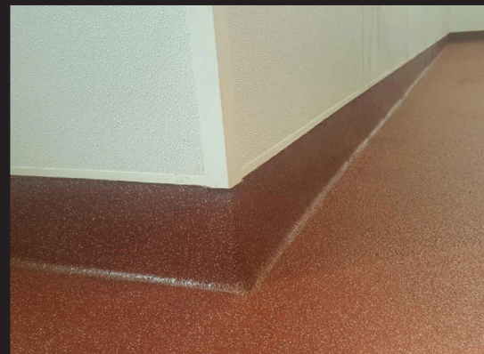
Integral 4" or 6" cove base creates a bathtub effect for effective waterproofing.
